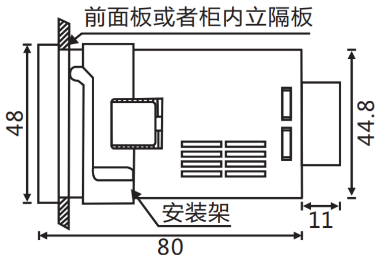
嵌入式外形与安装开孔尺寸 (开孔尺寸:45.5*45.5mm)
